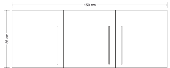
HS 150 - drawing
