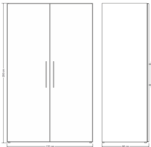
Drawing: SKM - Dimensions
