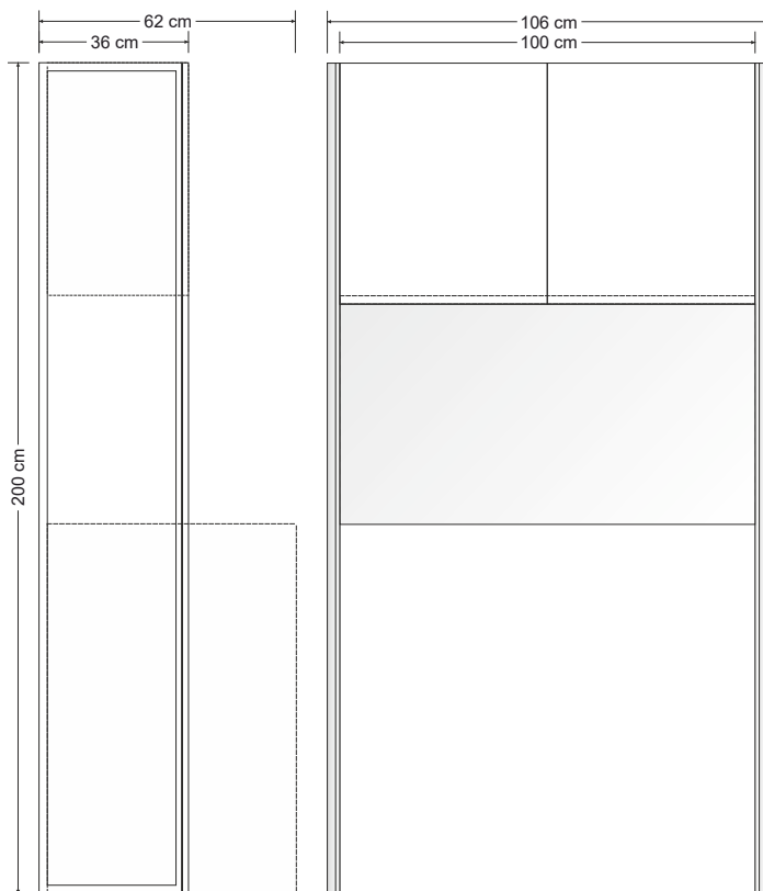
Studioline E drawing side
