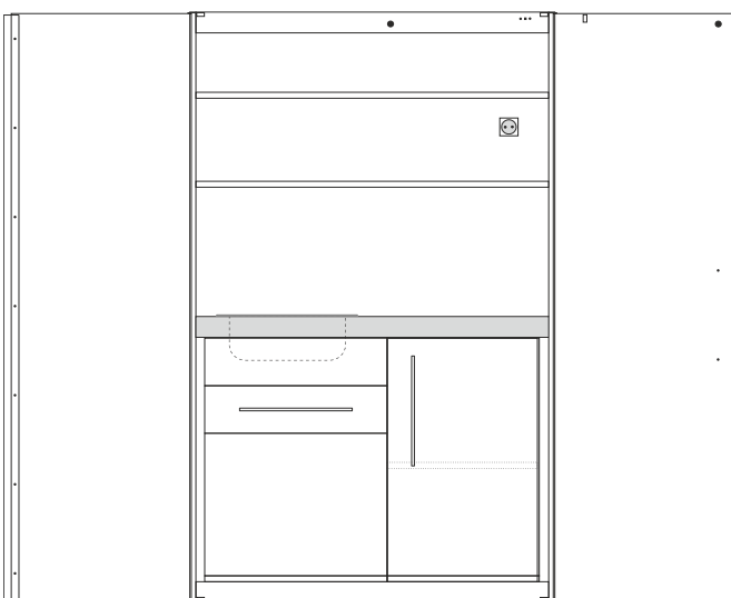
Drawing: SKM - Basic model without appliances
