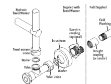
VALVE INSTALLATION
