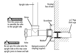
VALVE INSTALLATION
