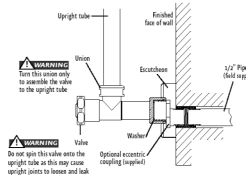
VALVE INSTALLATION
