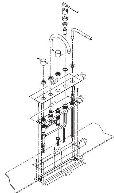
Paigaldamiseks otse vanni servale (BKB System)
